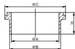
焊接接头 Welding Liner BS4825 PART 4 IDF-14
