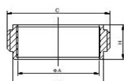
胀管云头 Expanding Male BS4825 PART 4 IDF-15R
