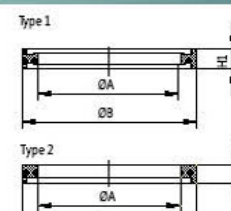
密封圈 Seal Ring BS4825 PART 4
