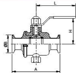
无滞留两通球阀 Non-Retention Straight Ball Valve DIN
