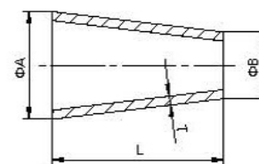
Concentric reducer RK
