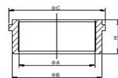
胀管接头 Expanding Liner BS4825 PART 4 IDF-14R
