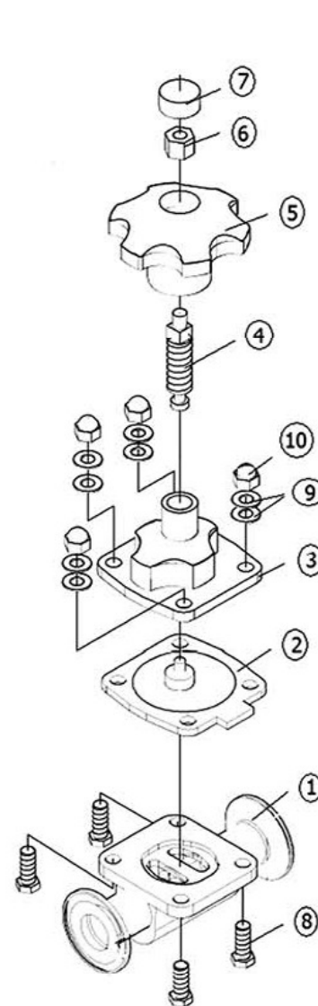
卫生级隔膜阀 Sanitary Diaphragm Valve
