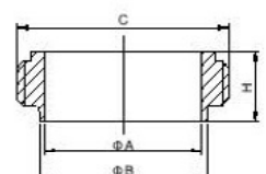
焊接云头 Welding Male BS4825 PART 4 IDF-15
