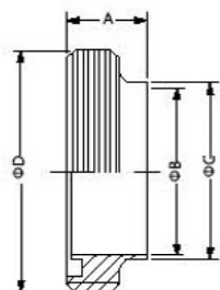
焊接云头 Welding Male
