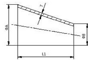
Eccentric reducer RE
