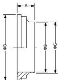
焊接接头 Welding Liner
