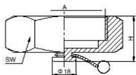
带耳六角盲盖 Hexagonal Blank Nut with Boss BS4825 PART 5 RJT-13HBN
