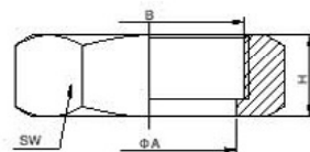
六角螺帽 Hexagonal Nut BS4825 PART 4 IDF-13H
