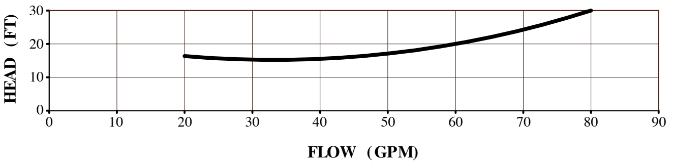
NPSHR (4" Impeller)
