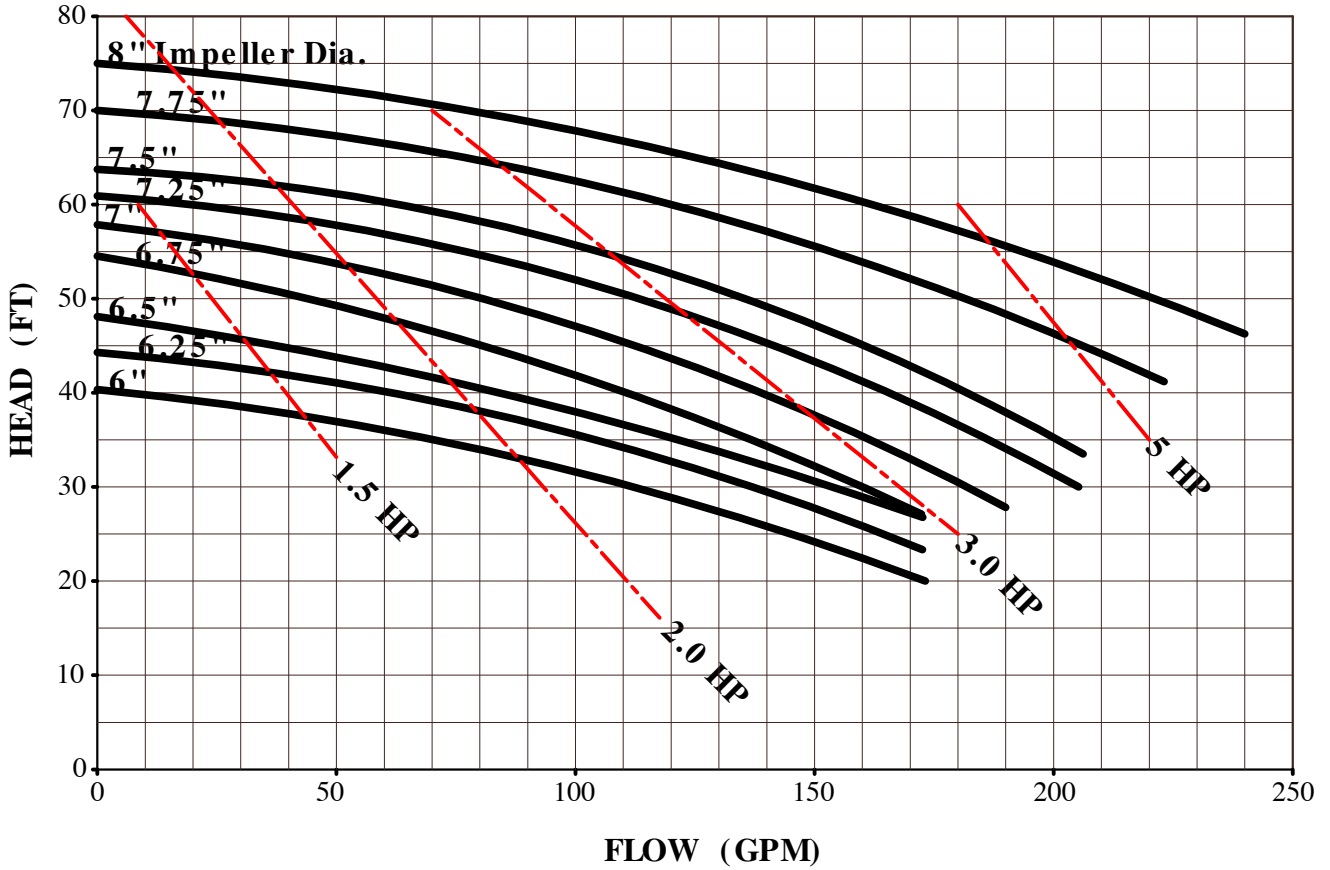
C318 @ 1750 RPM
