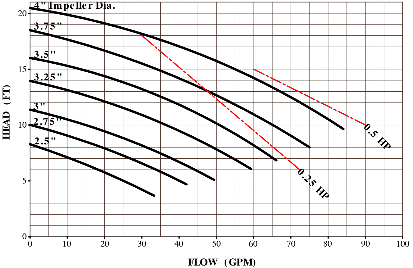
C114 @ 1750 RPM
